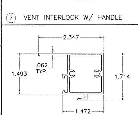
⑦ VENT INTERLOCK W/ HANDLE
