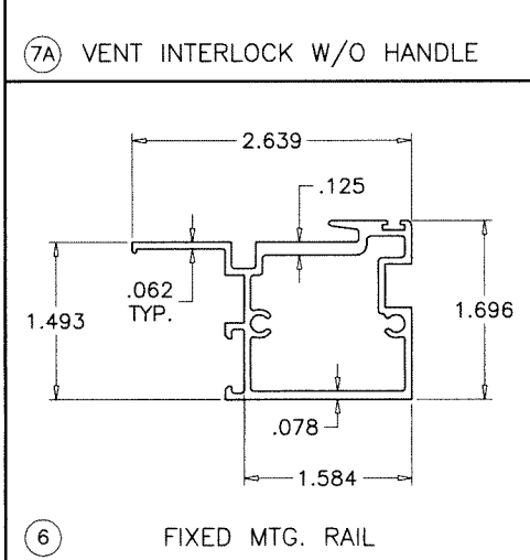
7A VENT INTERLOCK W/O HANDLE
